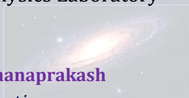
M31 - Andromeda Galaxy
